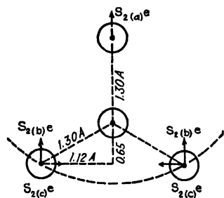
FIG. 4.—Diagram of \text{CO}_3^- group. The electric vector is parallel to the line joining the carbon to one of the oxygens (ordinary ray for calcite). (Bragg.)
